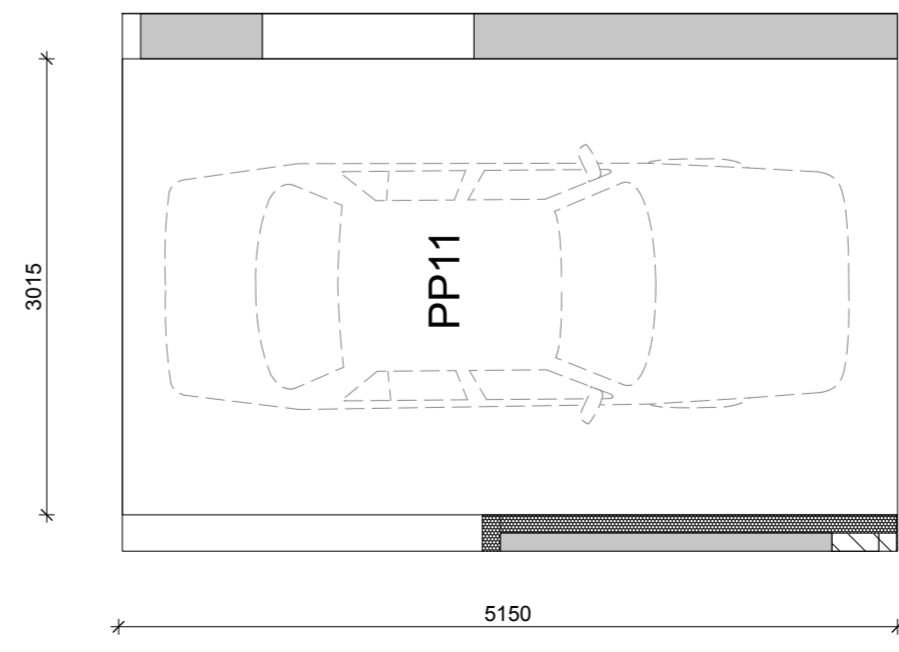
stallingsgarage
